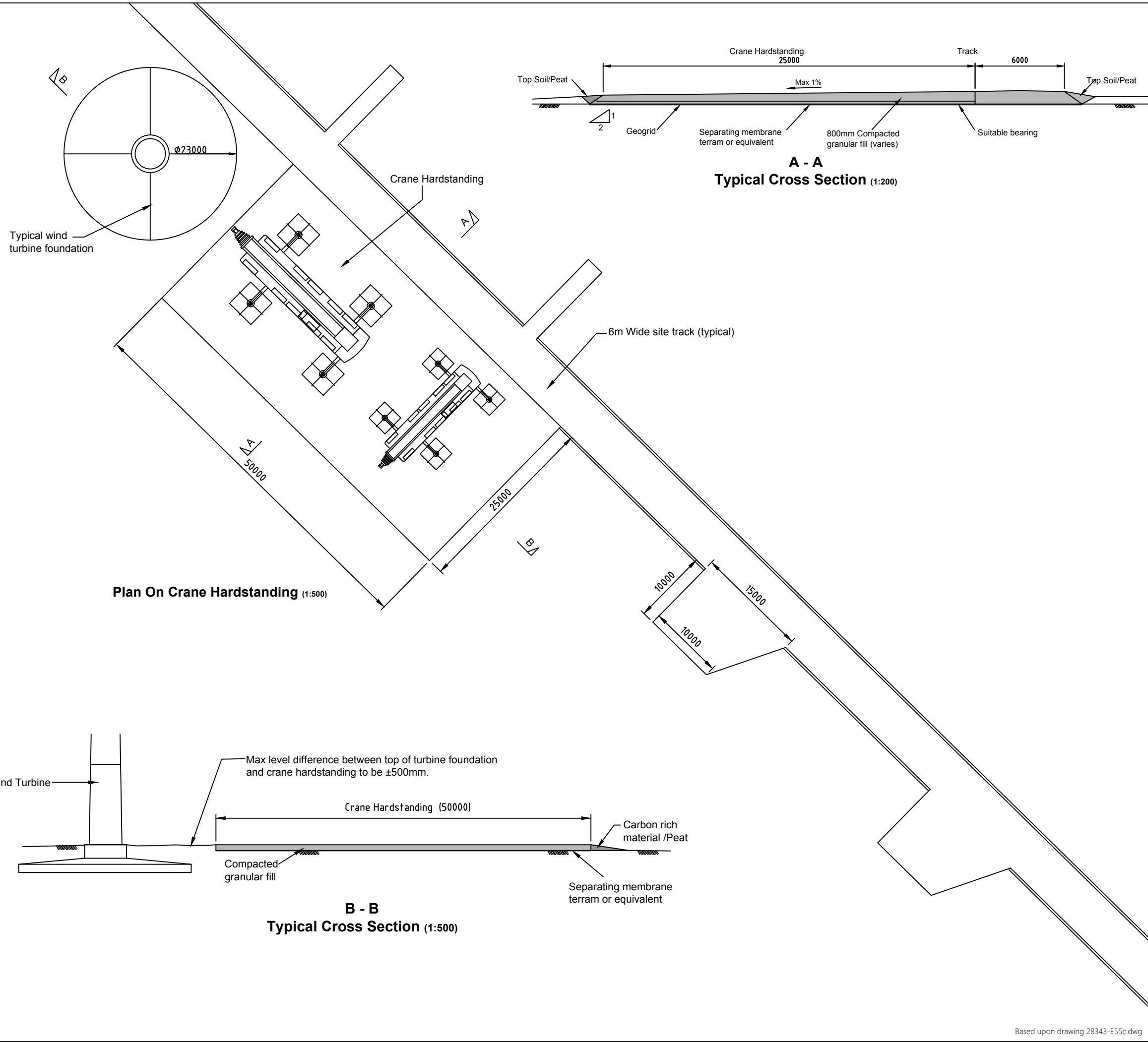
Figure 4.5 Typical crane hardstanding
