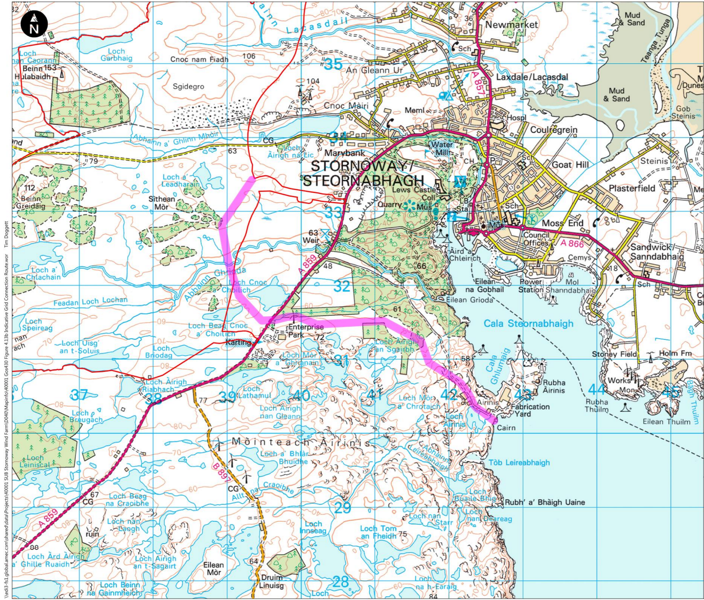
Figure 4.13 Indicative Grid Connection Route
