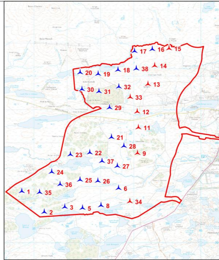
Layout 3 - Design Day Layout S9 (35 turbines)
