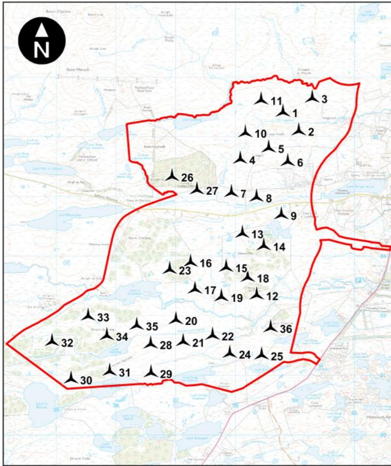
Layout 1 - Consented Layout (36 turbines)
