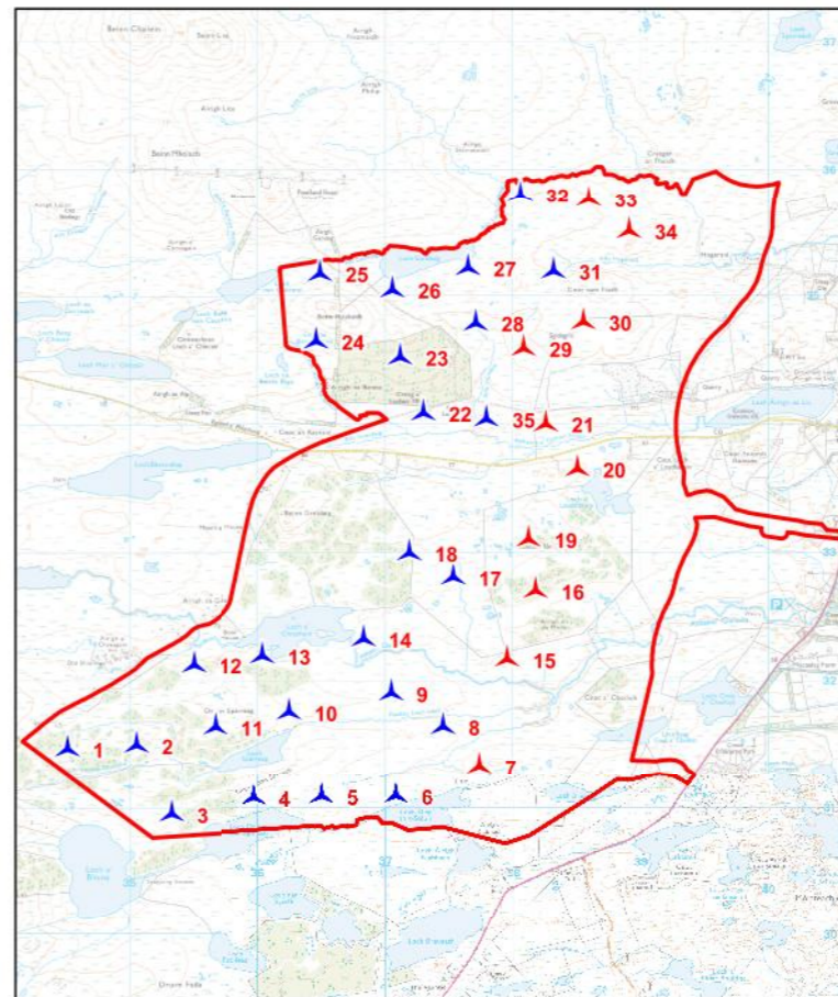
Layout 6 - EIA Layout (35 turbines)
