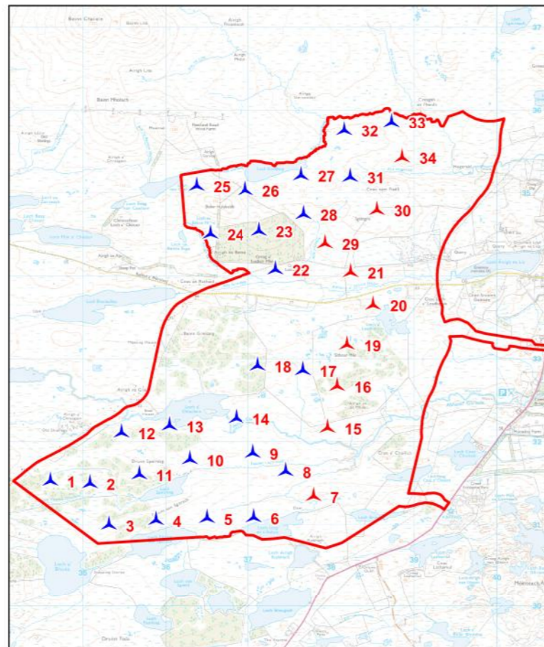
Layout 5 - S12 Layout (34 turbines)
