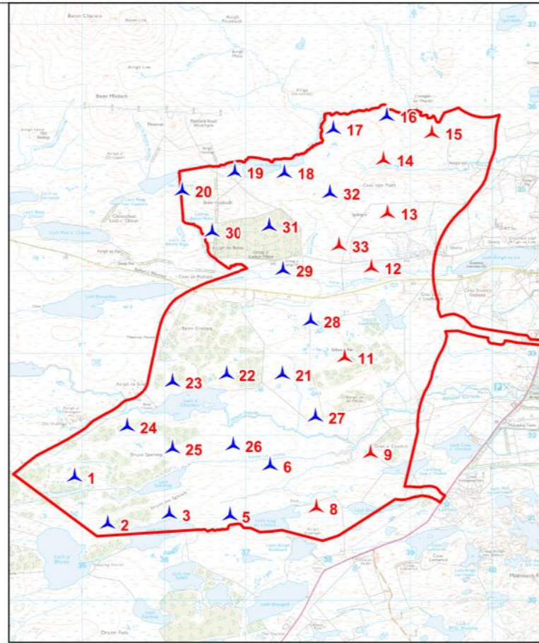
Layout 2 - S6 Layout (30 turbines)
