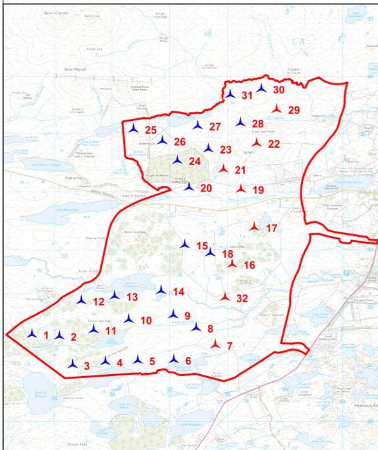
Layout 4 - S11 Layout (32 turbines)
